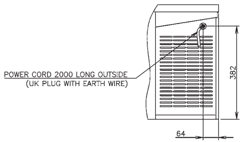
VIEW A (1/10)
